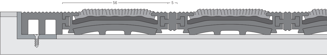
Typical installation example: Interior entrance, closed construction, 12mm aluminium base, Boulevard 5000 wiper, EPES4012 edging strip with UMFA12 recessed frame
